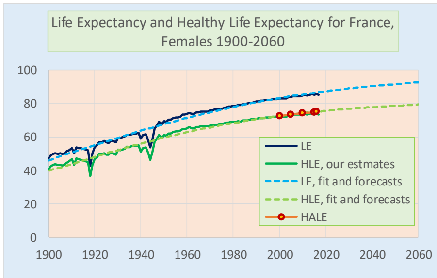
Fig. 3. Logistic model fit and forecasts to 2060 for females in France.
