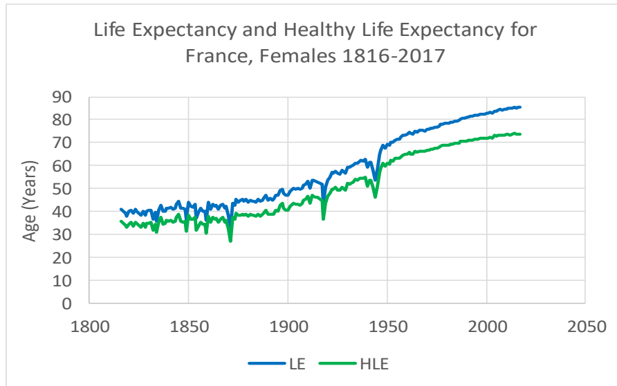
Fig. 1. Life Expectancy (LE) and Healthy Life Expectancy (HLE) in France, females (1816-2017).
